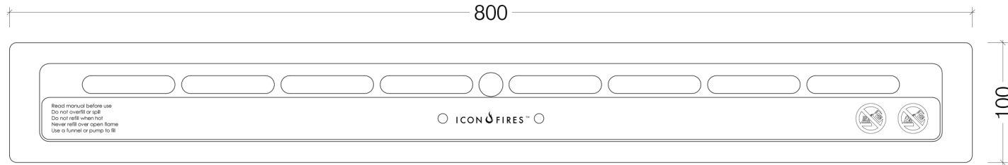
Top View
